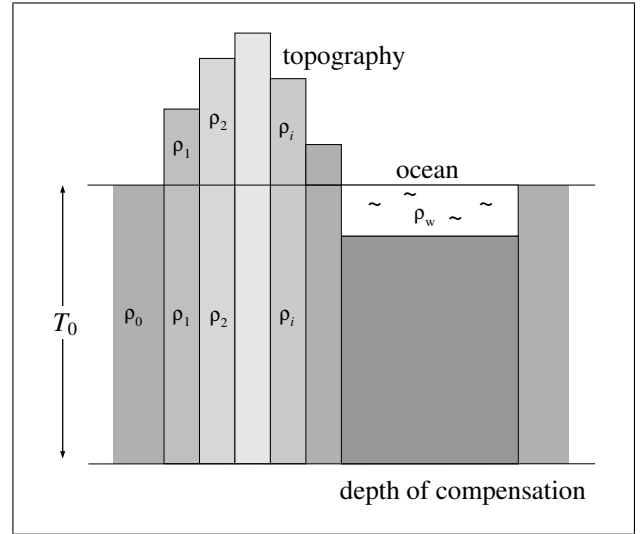
Figure 8.7: Pratt-Hayford model: constant depth of compensation T_0 and variable column density \rho_i .
