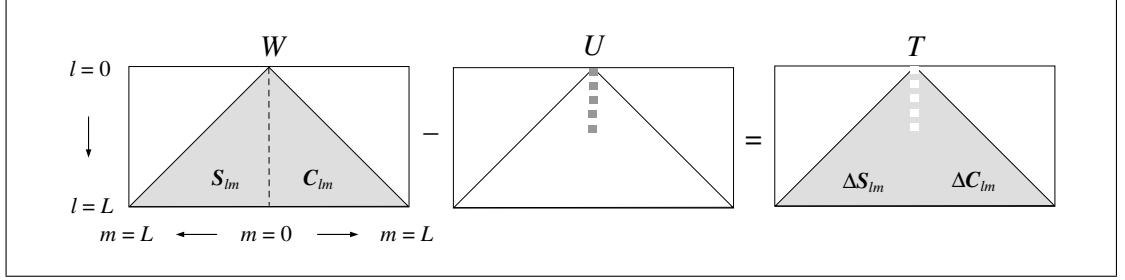
Figure 8.1.: Subtracting the normal potential U from the full gravity potential W in the spectral domain yields the disturbing potential T .
