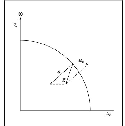
Figure 4.1: Gravity is the sum of gravitational attraction and centrifugal acceleration. Note that \mathbf{a}_c is hugely exaggerated. The centrifugal acceleration vector is about 3 orders of magnitude smaller than the gravitational attraction.
